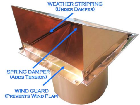
COPPER WIND DEFENDER VENT
