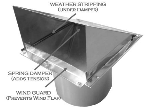
STAINLESS WIND DEFENDER VENT
